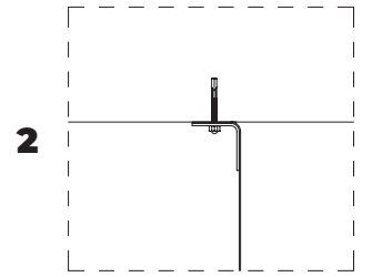
CONCRETE STEEL ANCHOR DETAIL
