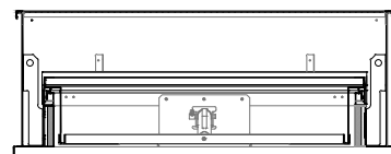
SECTION S1
