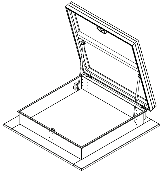
PERSPECTIVE VIEW
