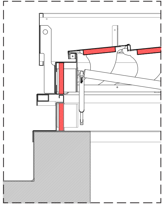
DETAIL 02 double wall aluminium with insulation
